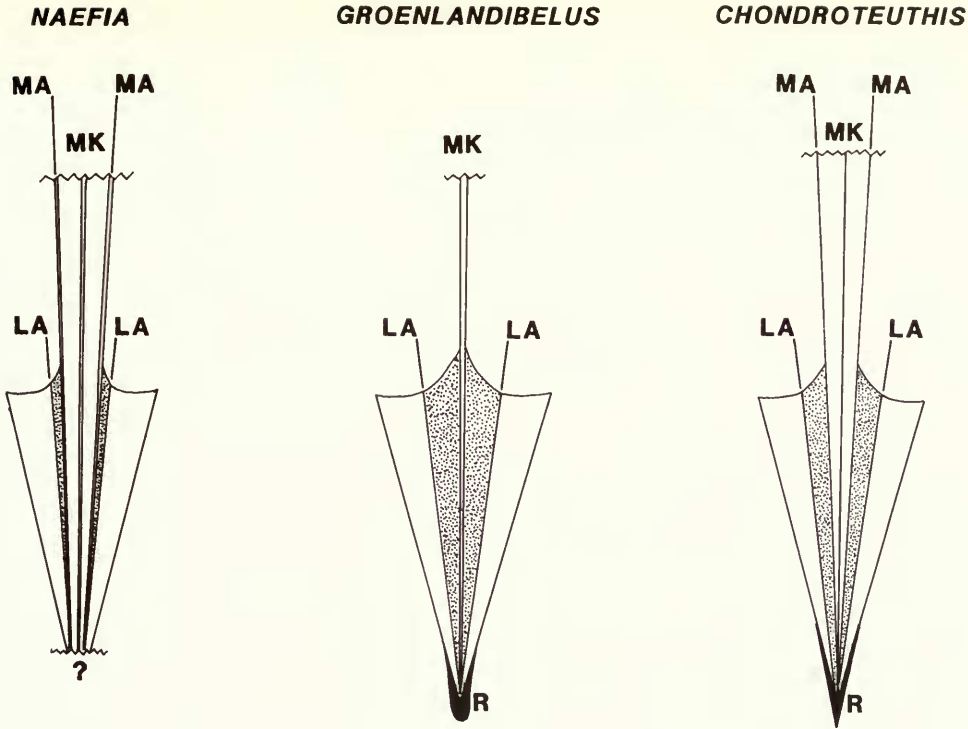
Fig. 5 Schematic comparison of the phragmocones and pro-ostraca of Naefia , Groenlandibelus and Chondroteuthis , not to scale. Stipple, hyperbolar zones; R, rostrum. Other symbols as given in Fig. 4.
